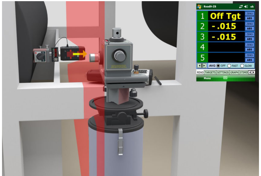
Adjusting the post length for A-1519-2.4ZB Targets in mag base so it can detect the laser.
