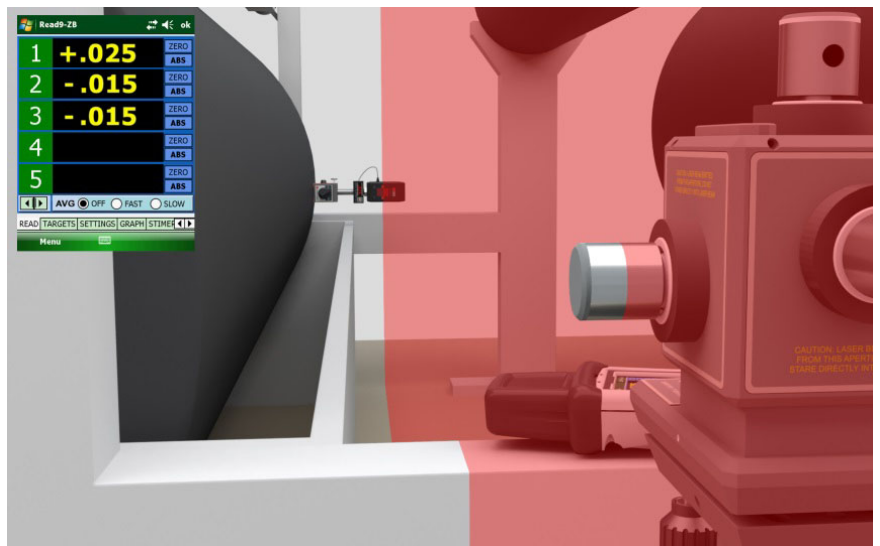
A-1519-2.4ZB Measuring Target at the far end of the roll measuring the parallelism
