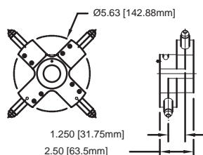
A-514B Target Adapter
