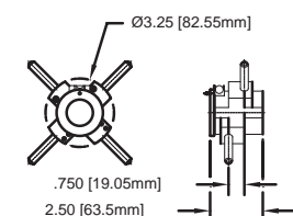
A-514A Target Adapter
