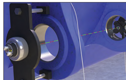
L-706 Laser Mounted in Boring-Bar Bearing
