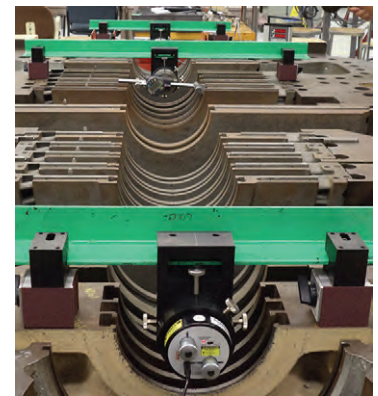
The L-706 Laser can be combined with our T-218T Turbine Target, half-bore fixtures and a bore sweep unit to make it the ideal system for aligning steam turbines
