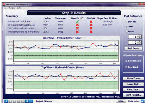
Bore9 Software showing plot of bore straightness.
