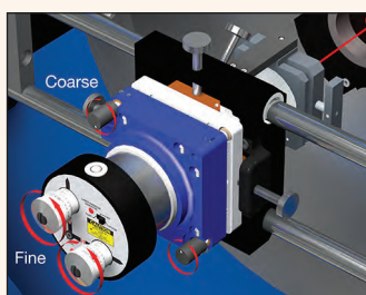
Adjusting Laser Angle with L-111 and L-706
