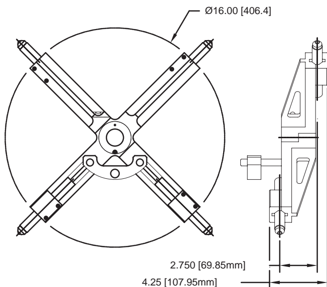
A-514C Target Adapter
