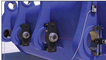
L-706 Aligning Boring-Bar Bearings in Bucket Loader
