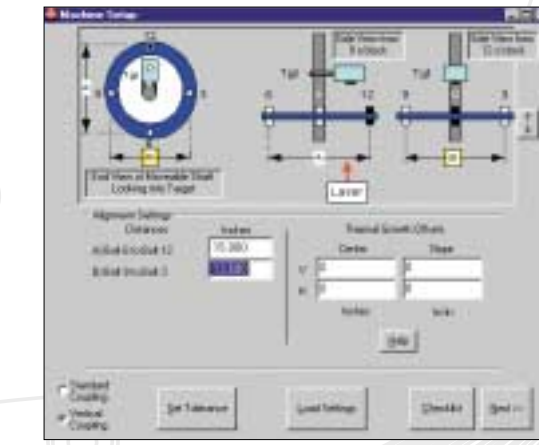
Vertical Pump Setup Screen. Enter the dimensions, tolerances and thermal offsets for accurate calculation of vertical pump shim values and moves.
