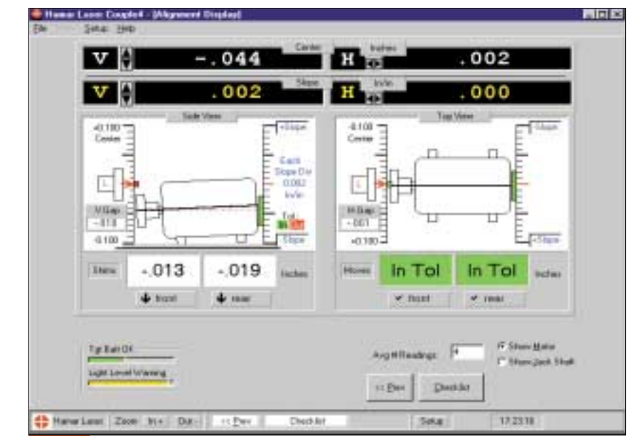
Step 5 Provides shim values, horizontal moves and a live alignment status for all 4 axes simultaneously. Shim box turns green when alignment tolerances are met.
