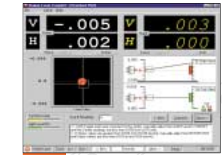
Step 2 Set up laser/target and adjust readings <0.030" and use for rough angular alignment on new installations.
