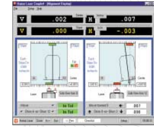
Vertical Pump Misalignment Screen. Provides shim values and moves for vertical pumps and a live 4-axis alignment status. Shim box turns green when alignment tolerances are met.
